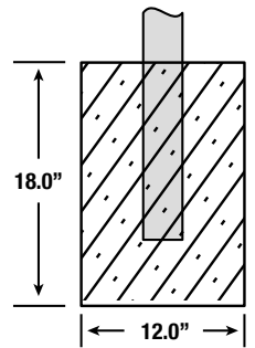
CONCRETE FOOTING
